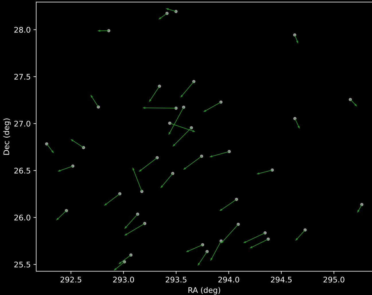
APOGEE DR17 Cluster 4 Proper Motion Vectors (n=38)
