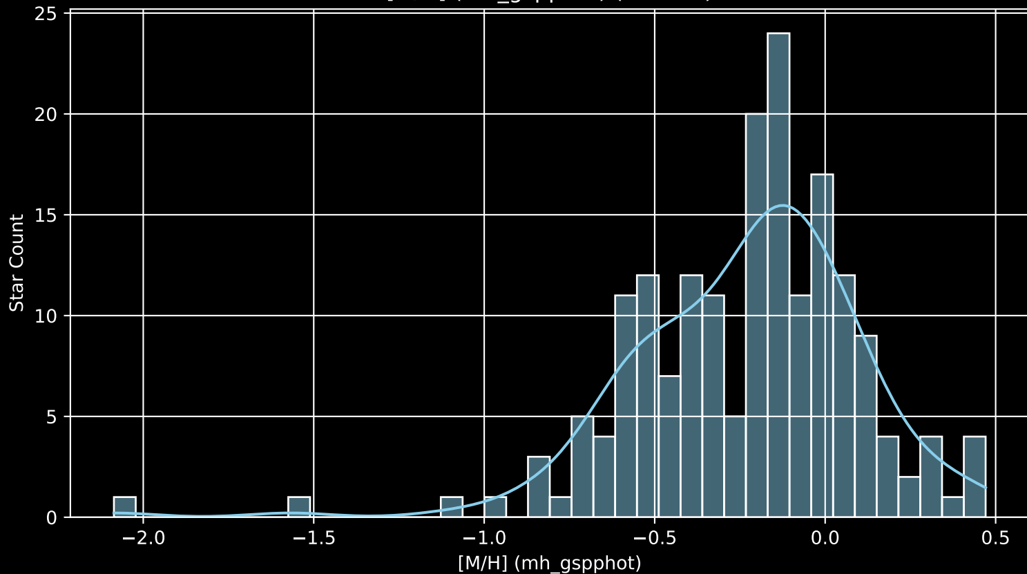
APOGEE DR17 Field: [014+89_MGA [M/H] (mh_gspphot) (n= 183)
