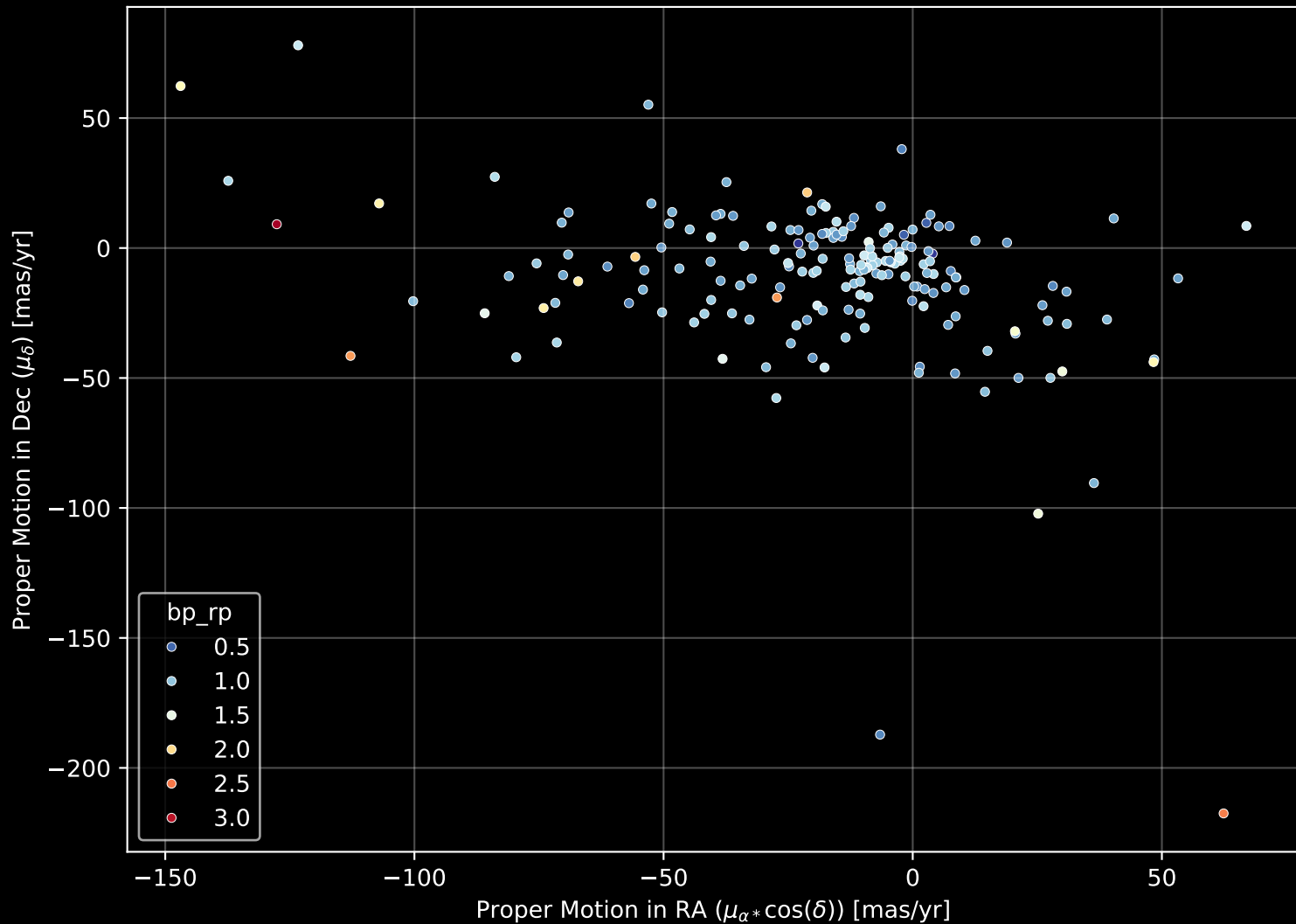
APOGEE DR17 Field: [014+89_MGA] Proper Motion Diagram (n= 185)
