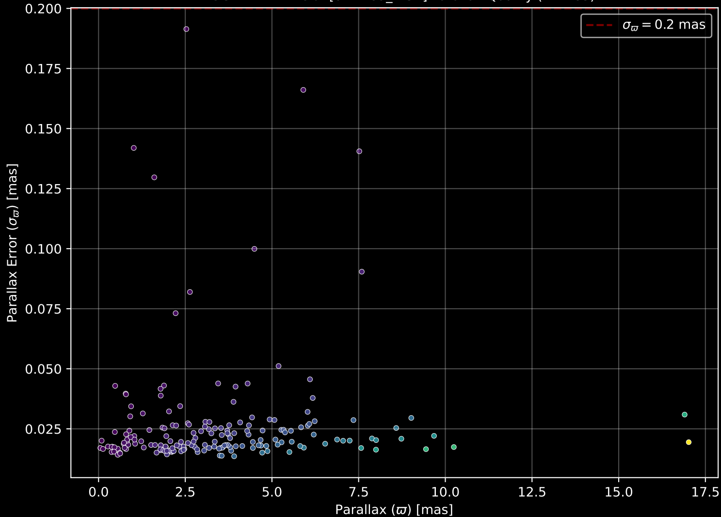
APOGEE DR17 Field: [014+89_MGA] Parallax Quality (n= 185)
