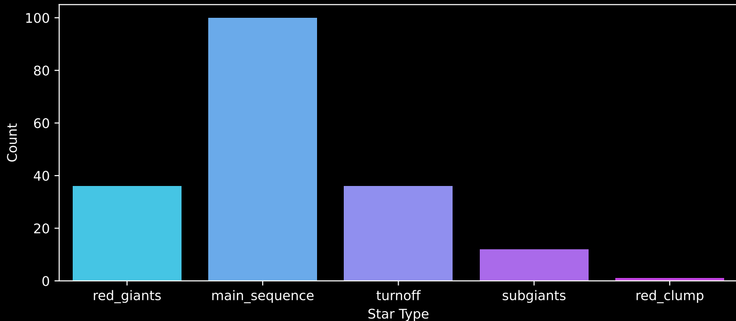
APOGEE DR17 Field: [014+89_MGA] Count plot of Star Type
