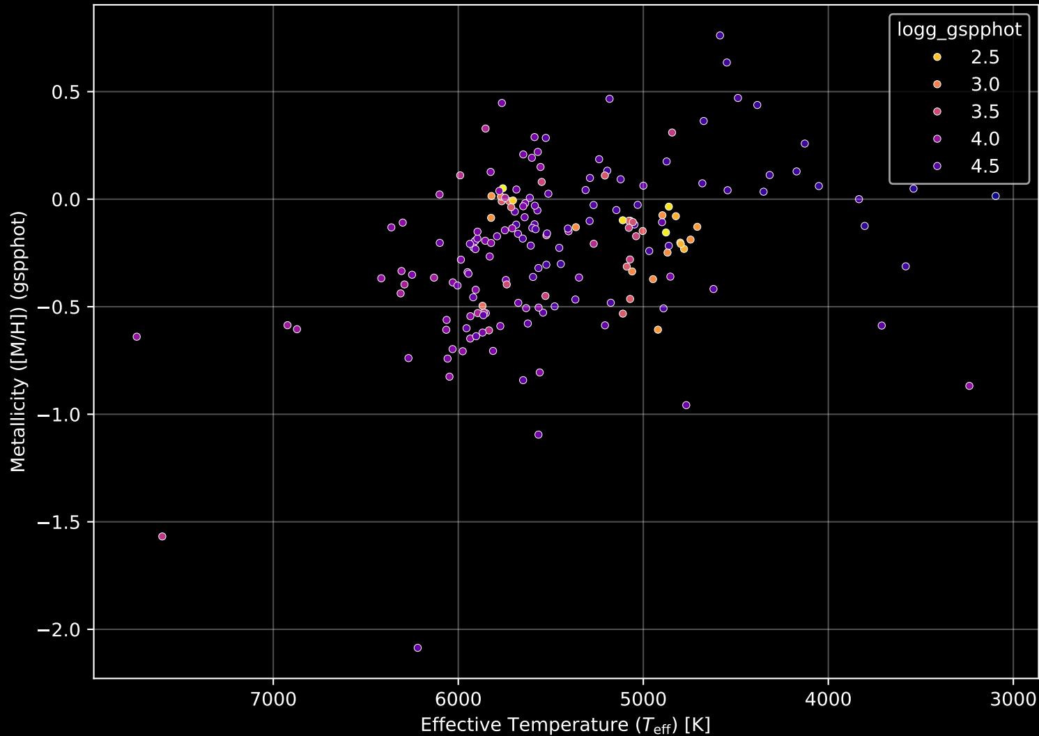
APOGEE DR17 Field: [014+89_MGA] Stellar Population Parameters (n= 185)
