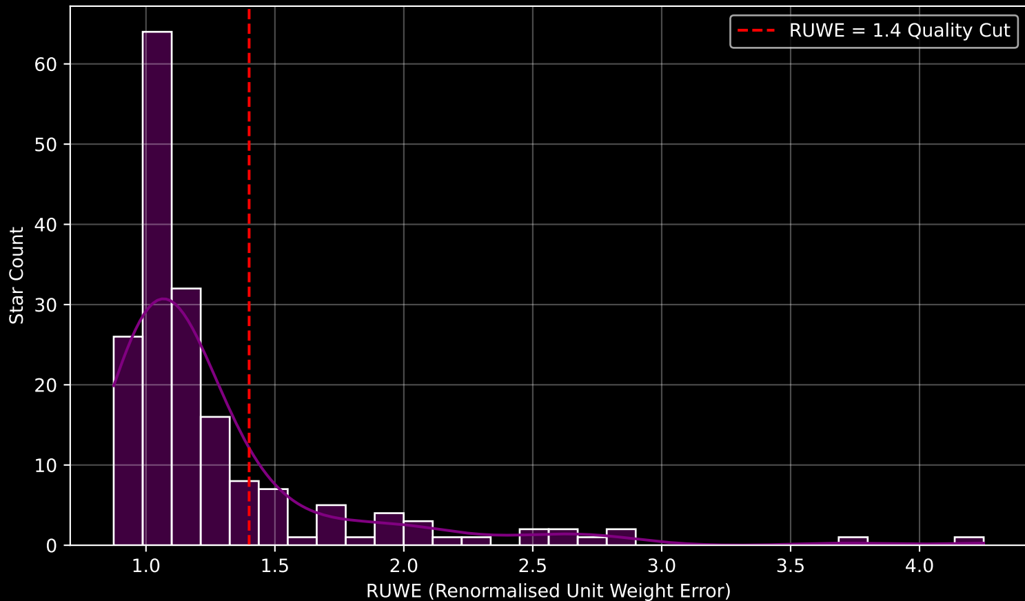
GAPOGEE DR17 Field [014+89_MGA] RUWE Distribution (n= 178)
